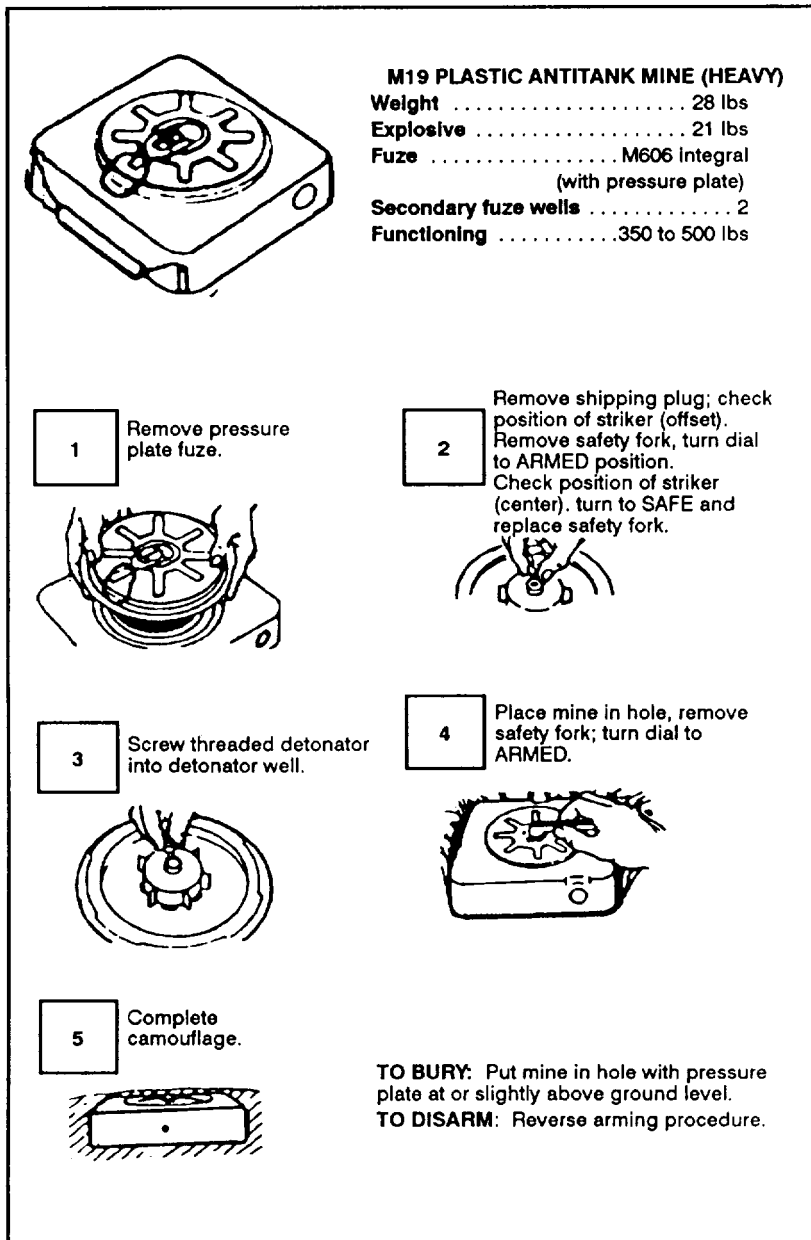
Figure B-9. Antitank mines (continued).
